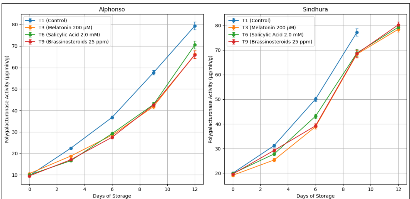
Fig. 2. Effect of bioactive compounds on polygalacturonase activity ( \mu\text{g}/\text{min}/\text{g} ) in mango varieties A) Alphonso and B) Sindhura under ambient storage. T_1 - Control (water dip); T_3 - Melatonin (200 \mu\text{M} ); T_6 - Salicylic acid (2.0 mM); T_9 - Brassinosteroid (25 ppm). Each value is a mean for 3 replicates ( p = 0.05 )
