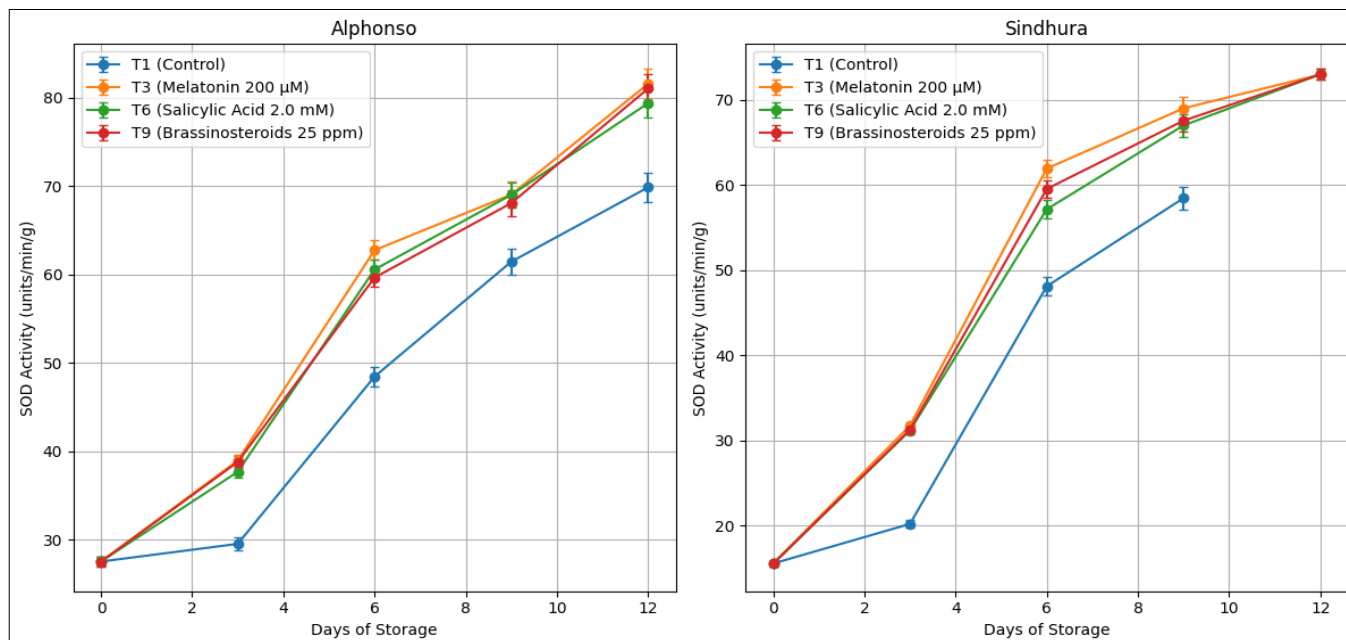
Fig. 7. Effect of bioactive compounds on superoxide dismutase activity (units/min/g) in mango varieties A) Alphonso and B) Sindhura under ambient storage. T 1 - Control (water dip); T 3 - Melatonin (200 µM); T 6 - Salicylic Acid (2.0 mM); T 9 - Brassinosteroid (25 ppm). Each value is a mean for 3 replicates ( p = 0.05 )
