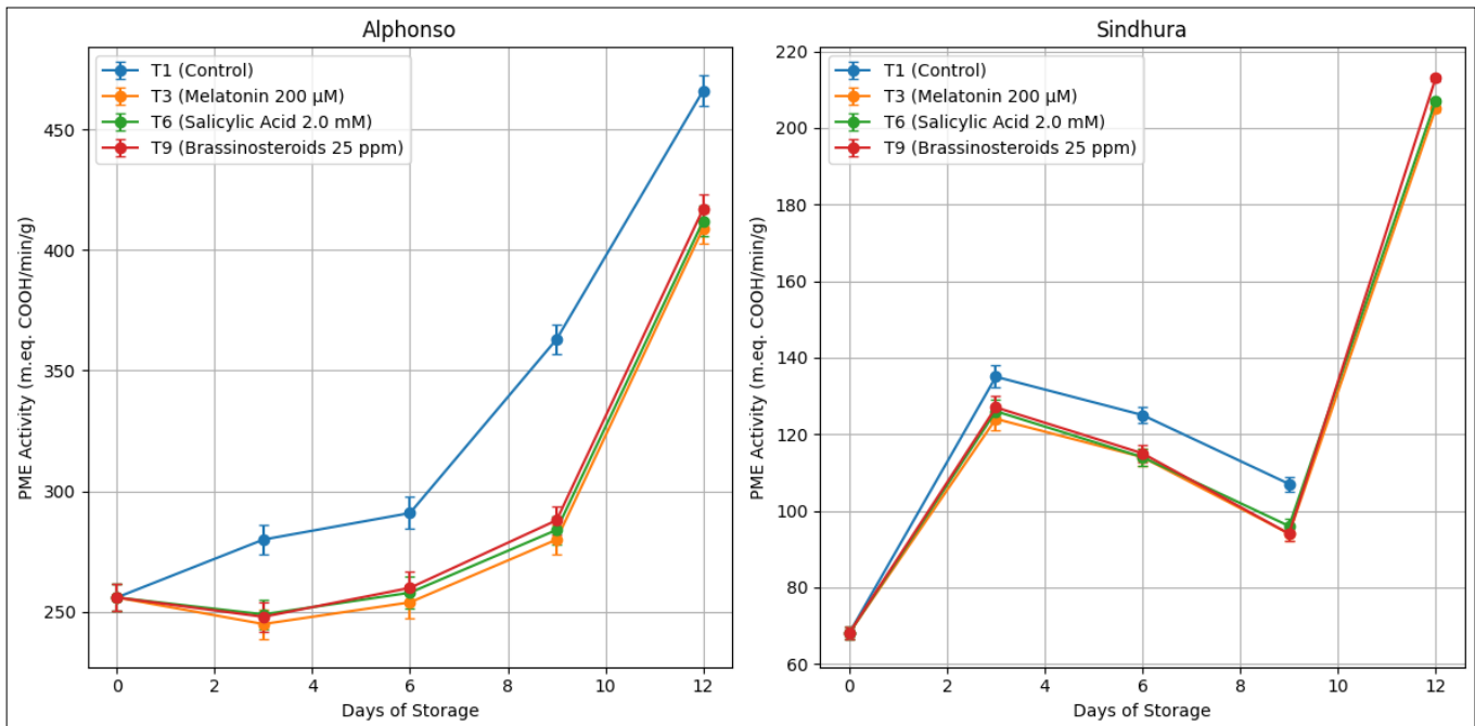
Fig. 1. Effect of bioactive compounds on PME activity (m.eq. COOH/min/g) in mango varieties A) Alphonso and B) Sindhura under ambient storage. T_1 - Control (water dip); T_3 - Melatonin (200 \mu\text{M} ); T_6 -Salicylic acid (2.0 mM); T_9 - Brassinosteroid (25 ppm). Each value is a mean for 3 replicates ( p = 0.05 )
