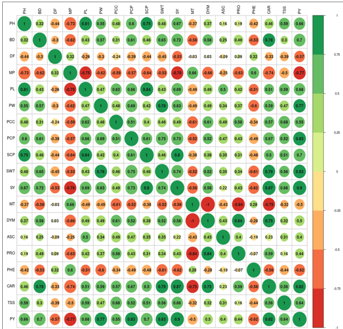
Fig. 1. Correlogram displaying the correlation coefficients of nineteen traits
