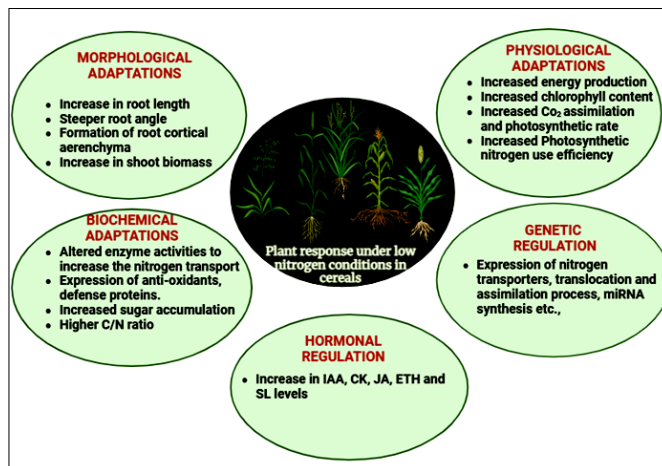
Fig. 2. Adaptations of cereals under low nitrogen conditions. \text{CO}_2 - Carbondioxide; C- Carbon; N- nitrogen; miRNA- microRNA; IAA- Indole acetic acid; CK- Cytokinin; JA- Jasmonic acid; ETH- Ethylene; SL- Strigolactones.
