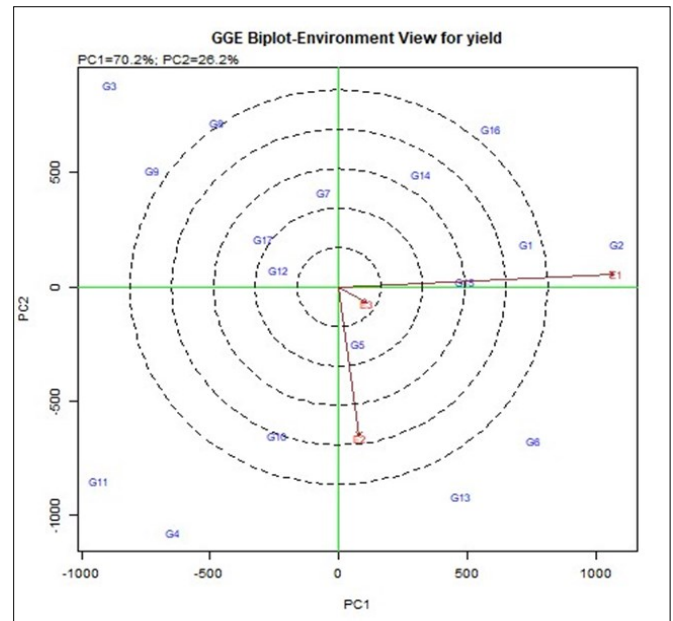
Fig. 5. Discriminativeness vs. representativeness pattern of GGE biplot.
