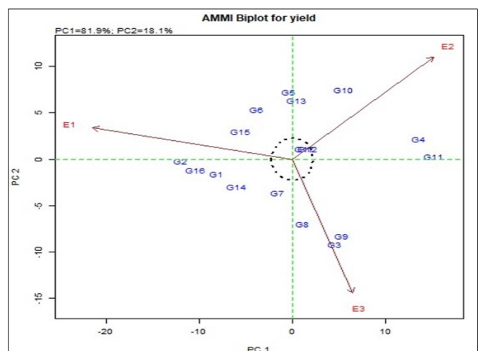
Fig. 2. AMMI 2 biplot for seed cotton yield.
