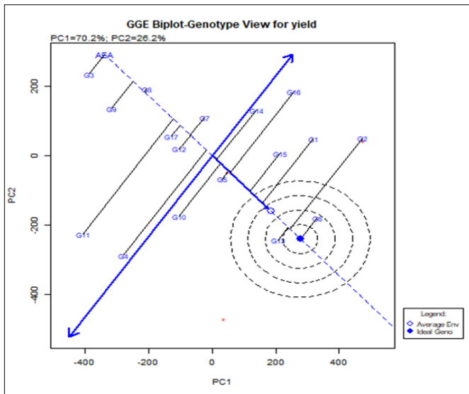
Fig. 4. Mean vs. stability pattern of GGE biplot.
