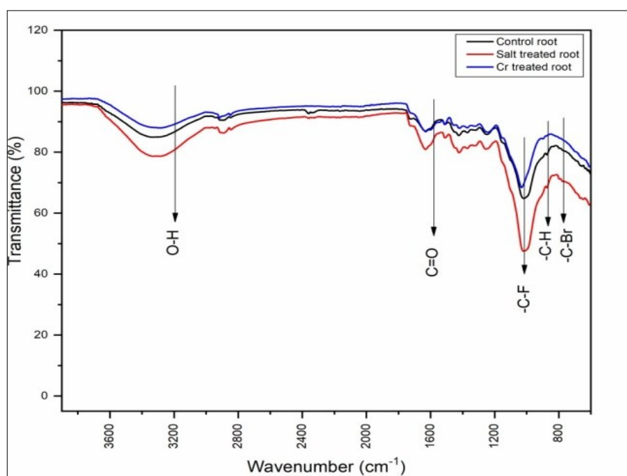
Fig.2. FTIR spectrum of vetiver root under different conditions
