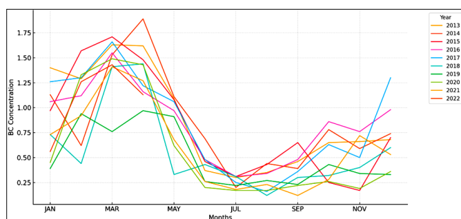
Fig. 6. Monthly variation of black carbon aerosol concentration from 2013 to 2023.
