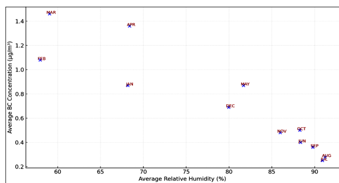
Fig. 8. Correlation between the BC concentration and relative humidity (2013–2023).
