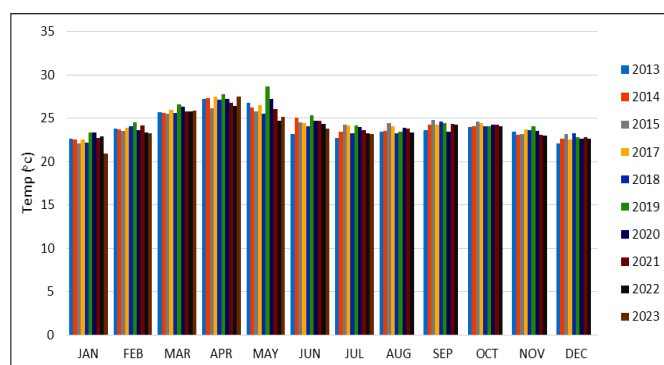
Fig. 2. Monthly variation of temperature over the years of 2013 to 2023.
