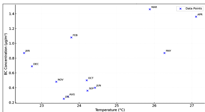
Fig. 7. Correlation between the BC concentration and temperature (2013–2023).
