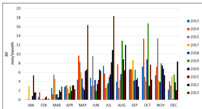
Fig. 4. Monthly variation of rainfall over the years of 2013 to 2023.
