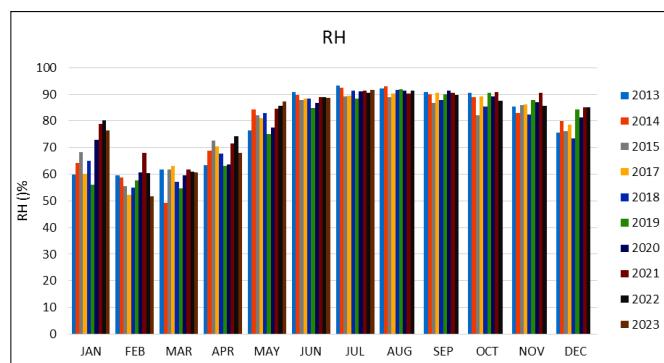
Fig. 3. Monthly variation of Relative humidity over the years of 2013 to 2023.
