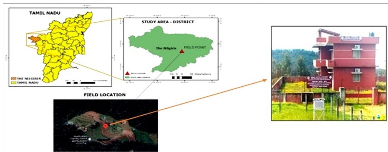
Fig. 1. ISRO-ARFI study site at Ooty, Tamil Nadu.
