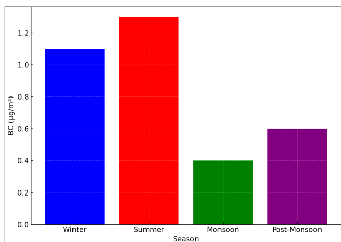
Fig. 5. Seasonal variation of black carbon aerosol concentration.
