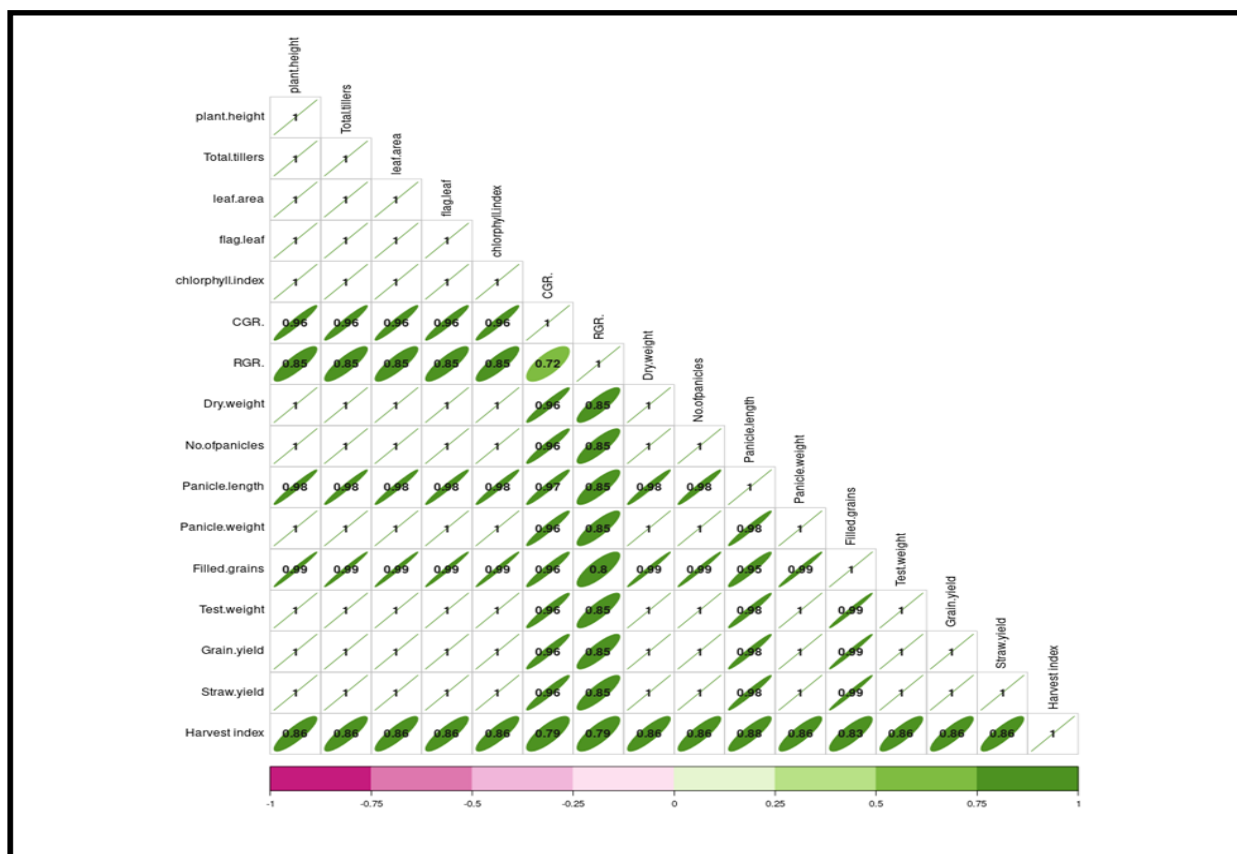
Fig. 3. Correlation matrix represented as a correlogram. It displays the correlation coefficients between different agronomic traits or variables measured in a study.
