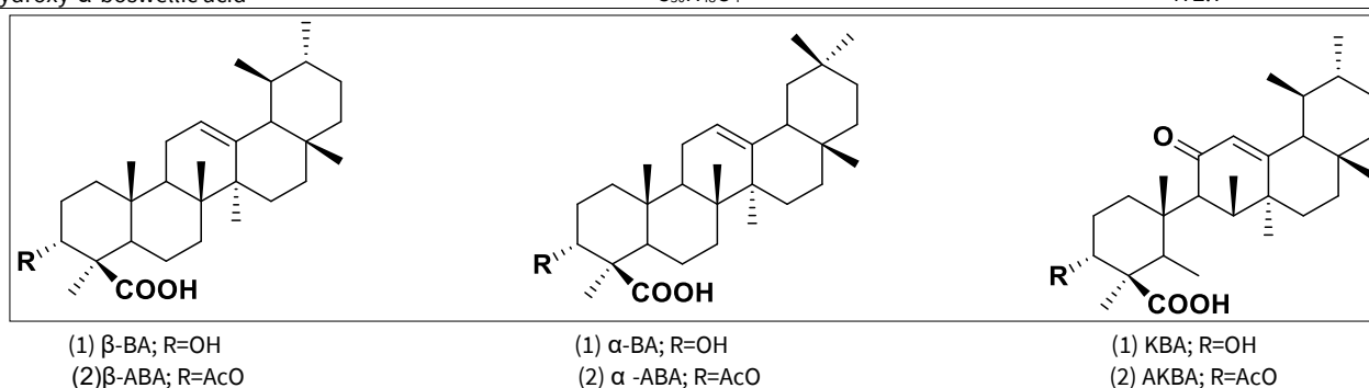
Fig. 1. Chemical structures of main BA.
