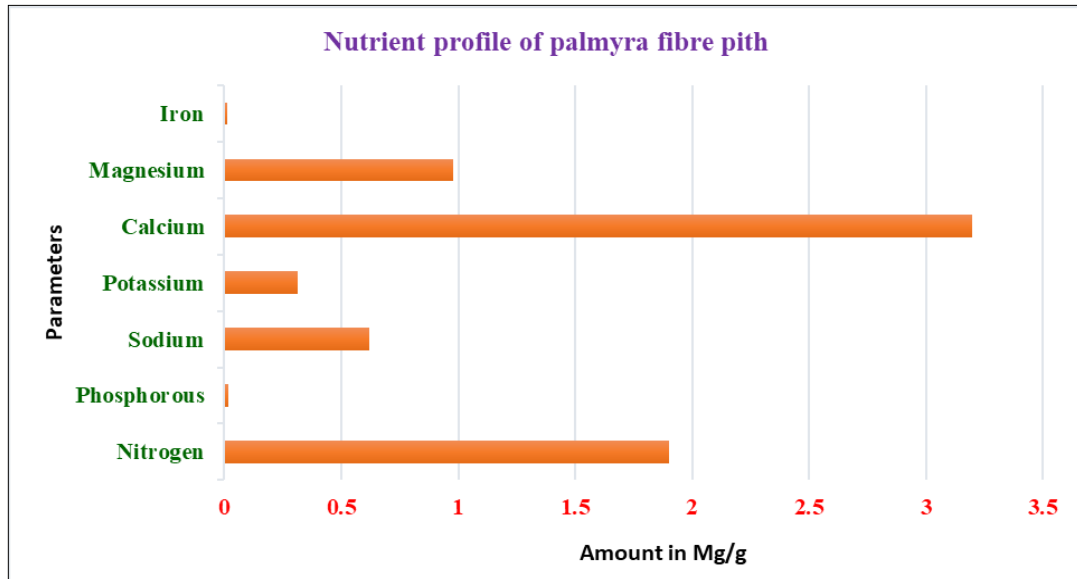
Fig. 3. Nutrient profile of palmyra fibre pith (58).
