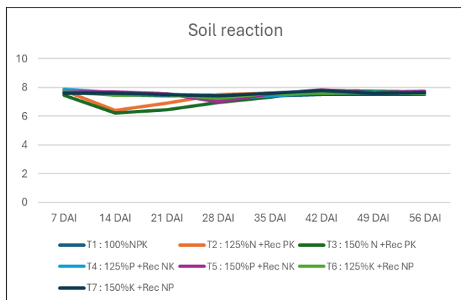
Fig. 1. Dynamic changing effect in soil reaction (pH) with varied levels of NPK fertilizers under submerged condition.
