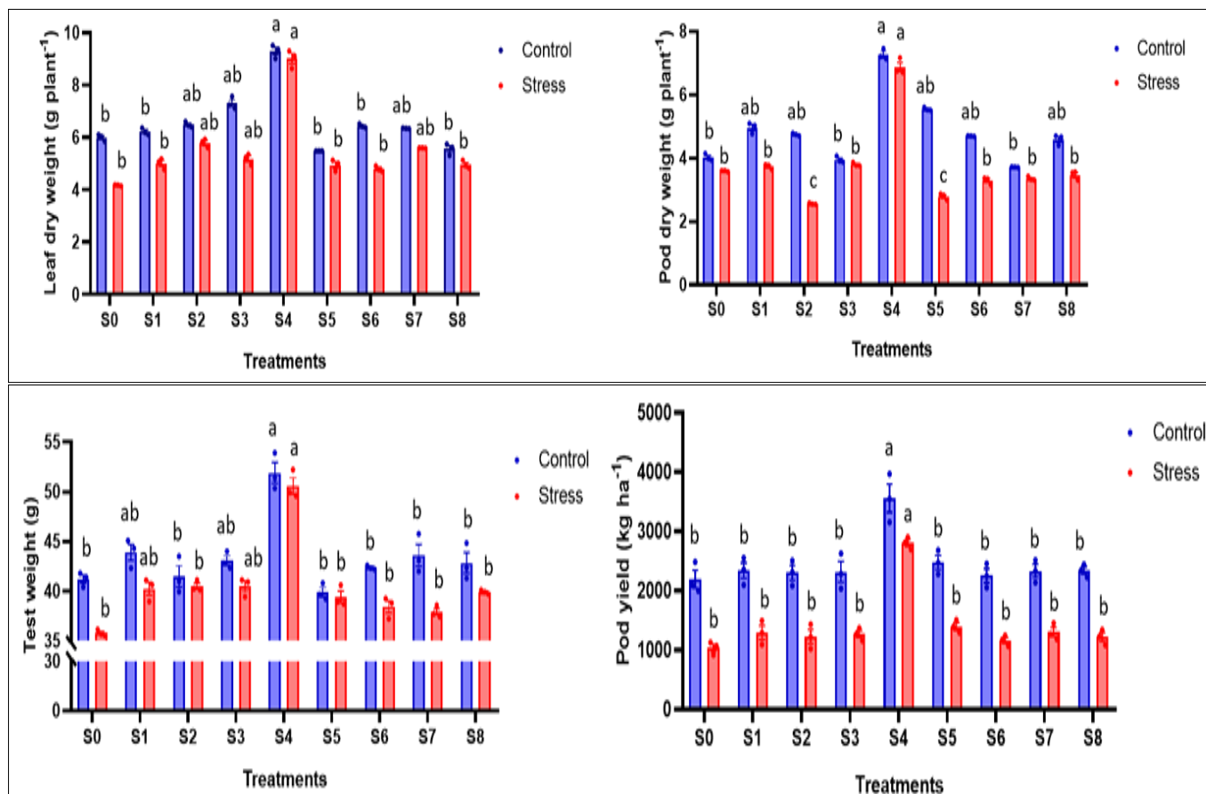
Fig. 1. Effect of signaling molecules on biomass partitioning in groundnut under water stress at 60 DAS (a) leaf dry weight (b) pod dry weight (c) test weight (d) pod yield. Here S0- Control, S1- ascorbic acid at 40 DAS, S2-ascorbic acid at 60 DAS, S3-salicylic acid at 40 DAS, S4-Salicylic acid at 60 DAS, S5-H 2 O 2 at 40 DAS, S6-H 2 O 2 at 60 DAS, S7- α-tocopherol at 40 DAS, S8- α-tocopherol at 60 DAS and DAS refers to Days after sowing. M1-Control, M2-Stress. This figure depicts the mean of three biological replicates and the statistical significance was tested using two-way ANOVA for split-plot design.
