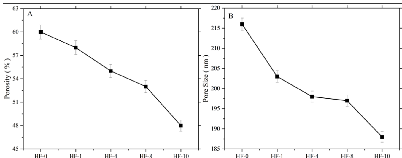
Fig. 5. Porosity (A) and pore size (B) performance test graphs of hemp-reinforced PA66 nanofiber membranes.
