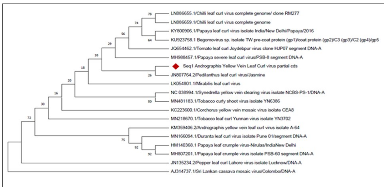
Fig. 5. Phylogenetic tree based on the nucleotide sequence of selected partial DNA-A, constructed using the NJ method in Clustal X and visualized in TreeView v1.6.5. Bootstrap values (100 replicates) are shown at the nodes. The DNA-A sequence associated with YVLCV used in this study is marked in red.
