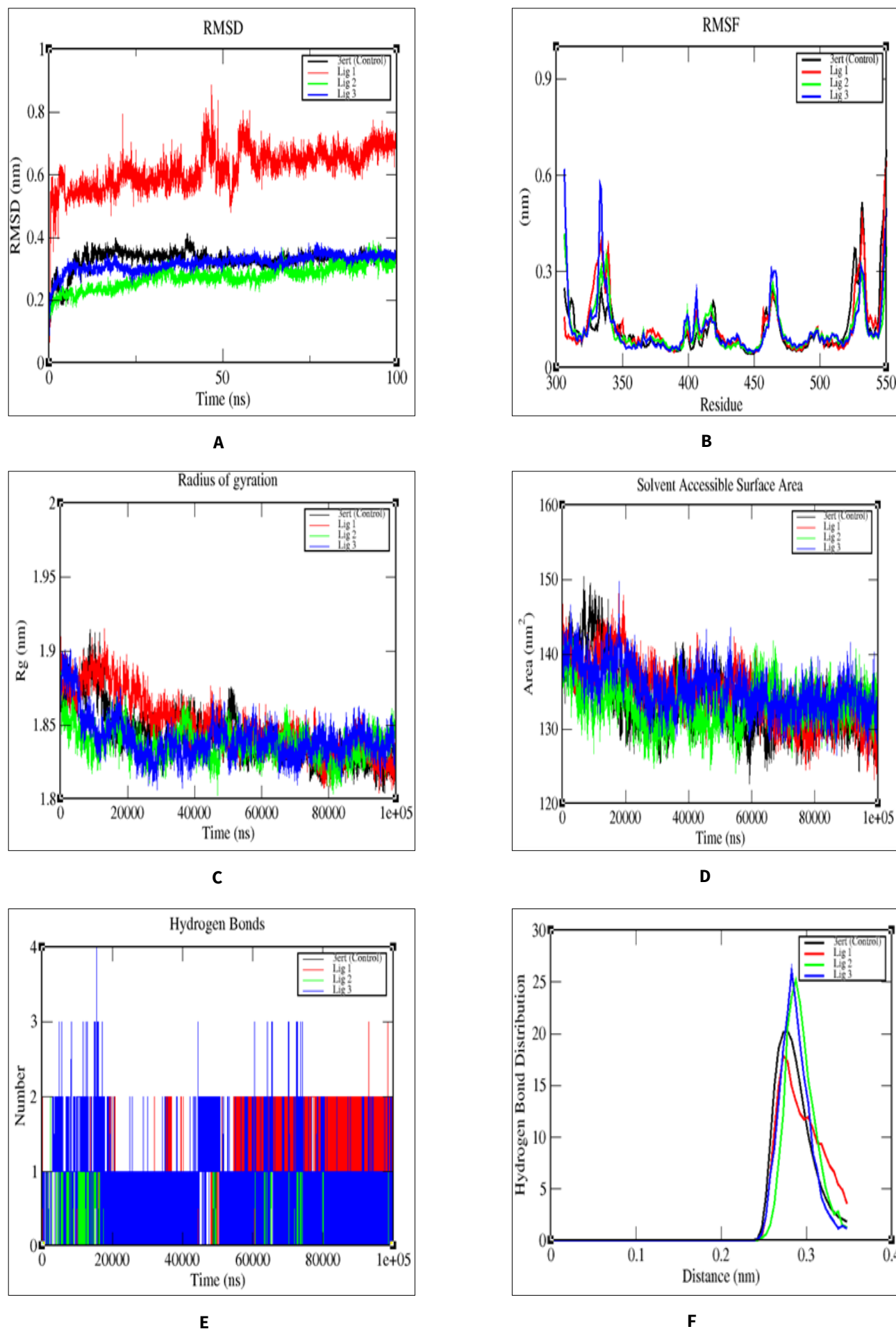
Fig. 4. Plot of MD simulation between L1, L2, L3 & ERα: (A) RMSD; (B) RMSF; (C) Radius of gyration; (D) SASA; (E) H-bond; (F) H-bond distribution.
