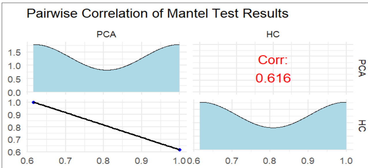
Fig. 7. Pairwise correlation between PCA and HC matrices using Mantel test (This figure illustrates the Mantel test correlation between distance matrices obtained from PCA and hierarchical clustering for the evaluated soybean germplasm. The lower-left scatter plot displays the relationship between the two distance matrices, showing a negative trend. The upper-left and lower-right density plots represent the distribution of distances within PCA and HC, respectively. The upper-right panel highlights the computed Mantel correlation coefficient ( r = 0.616 , p = 0.001 ) in red, indicating a moderate positive correlation between the two approaches despite the inverse trend in the scatter plot. This suggests that PCA and HC capture genetic divergence in different ways, reinforcing the robustness of genotype classification).
