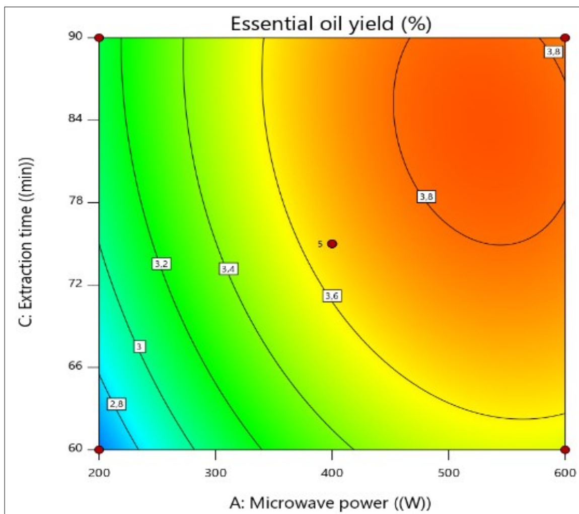
Fig. 3. 3D surface and contour plots of microwave power and extraction time of oil yield.
