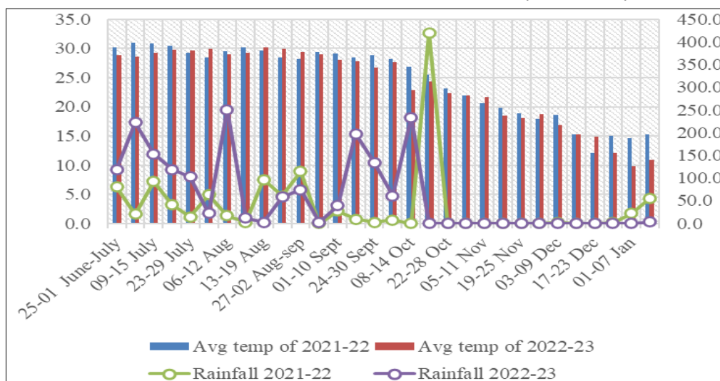
Fig. 1. Weekly weather data for the cropping season Rabi 2021-22 and Rabi 2022-23. Standard meteorological week on X-axis. Temperature on Y axis (left) and Rainfall on Y axis (right).
