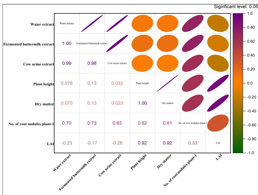
Fig. 4. Correlation matrix of organic extracts of seaweed and black gram growth parameters.
