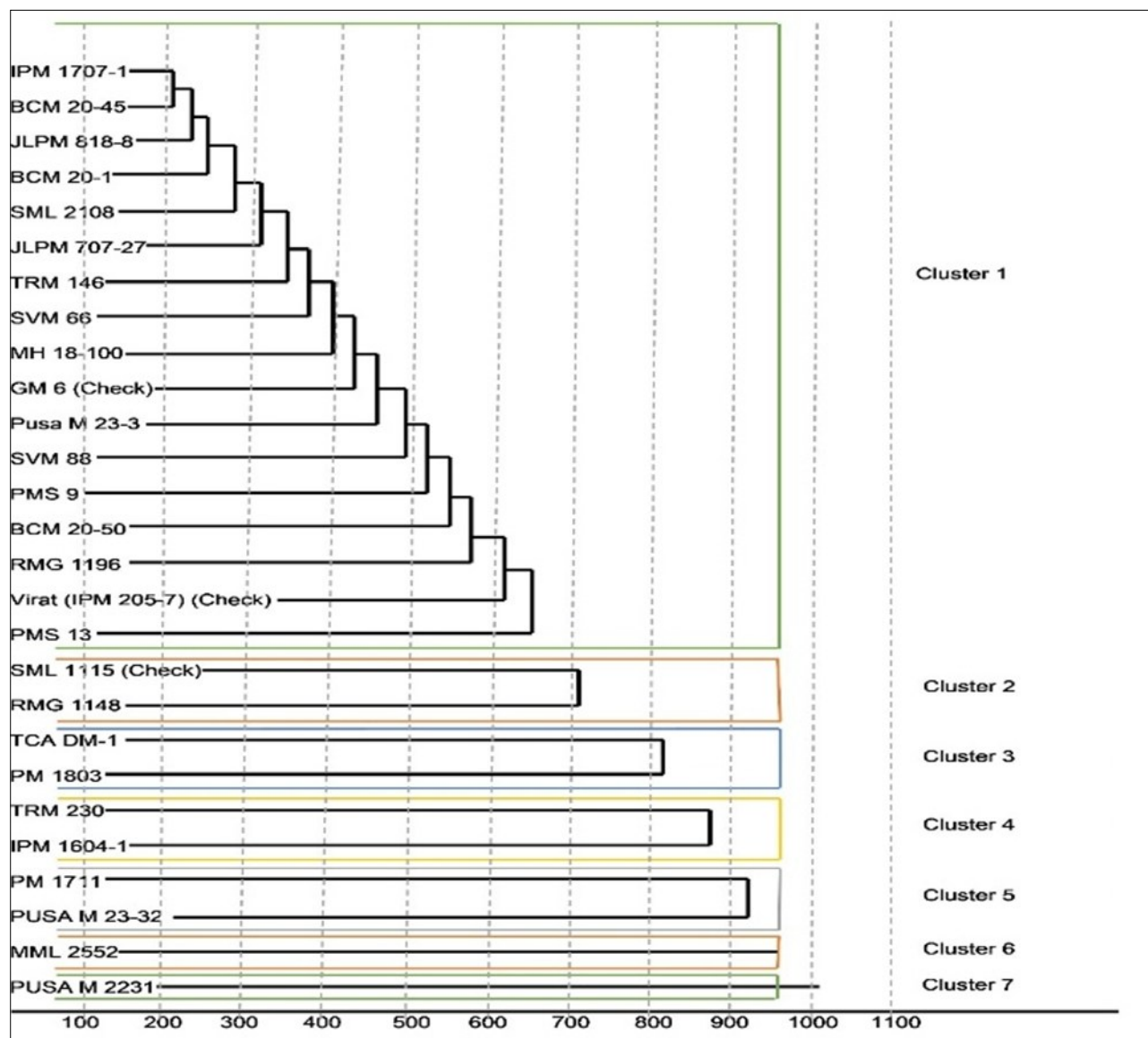
Fig. 1. Cluster dendrogram by Tocher's method.
