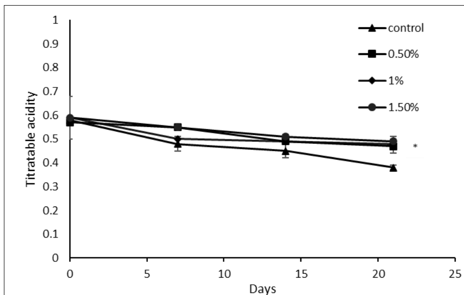
Fig. 6. Titratable acidity in CSM coated tomato fruits and uncoated fruits.
