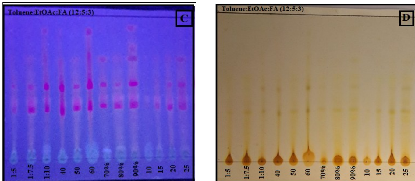
Fig. 3. Comparative TLC chromatograms for extracts obtained from a one-factor experiment at a time.
