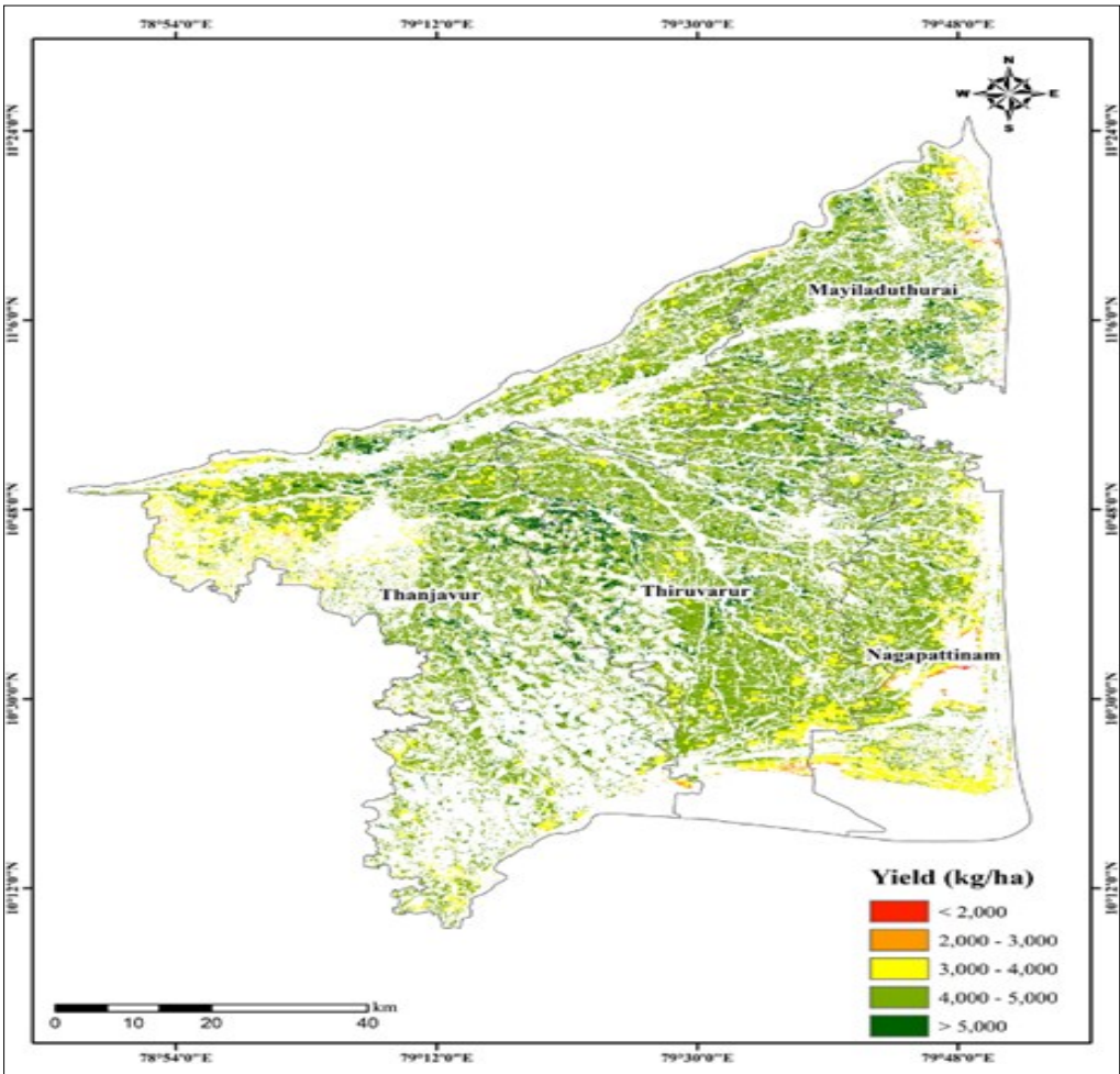
Fig. 7. Semi-physical model-based rice yield.
