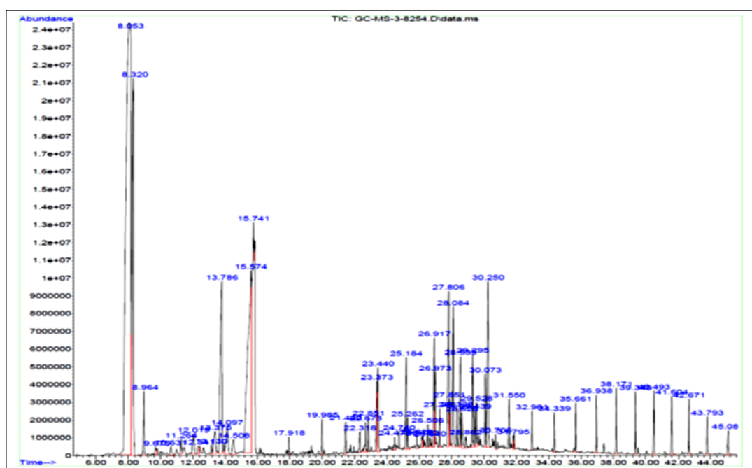
Fig. 1. Gas Chromatography-Mass Spectrometry chromatogram displays on essential oil composition from C. ambrosioides leaves.
