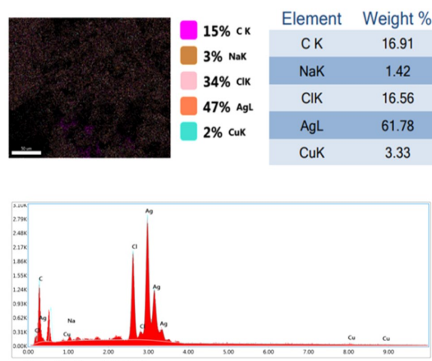
Fig. 4B EDS Spectrum of Ethanolic Leaf Extracts of C. fenestratum Containing Silver Nanoparticles (Ag NPs). This EDS (Energy-Dispersive X-ray Spectroscopy) spectrum presents the elemental composition of ethanolic leaf extracts from C. fenestratum containing synthesized silver nanoparticles (Ag NPs). The prominent peaks in the spectrum correspond to the characteristic X-ray emissions of the elements present. The presence of strong silver peaks confirms the existence of Ag NPs in the leaf extract. Additionally, other elemental peaks, if detected, may provide insights into the potential presence of additional elements, which could be attributed to the plant extract's phytochemical composition.
